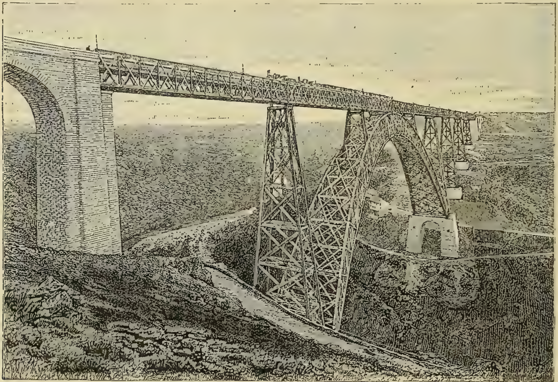
FIG. 4.—GENERAL VIEW OF THE VIADUCT OF GARABIT.
